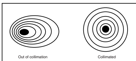
Figure 15. A star test will determine if the telescope's optics are properly collimated. An unfocused view of a bright star through the eyepiece should appear as illustrated on the right if optics are perfectly collimated. If the circle is unsymmetrical, as illustrated on the left, the scope needs collimation.
