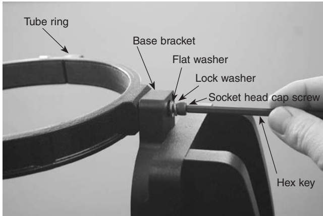
Figure 3. Attaching a tube ring to the base bracket.
