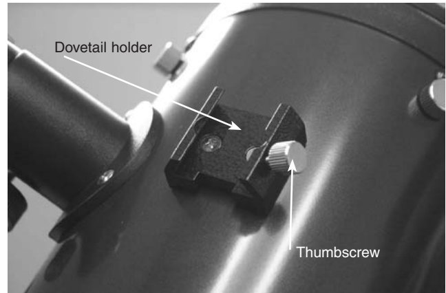
Figure 4. The EZ Finder II dovetail holder.
