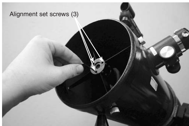
Figure 12. Adjust the tilt of the secondary mirror by loosening or tightening the three alignment set-screws with a 2mm hex key.
