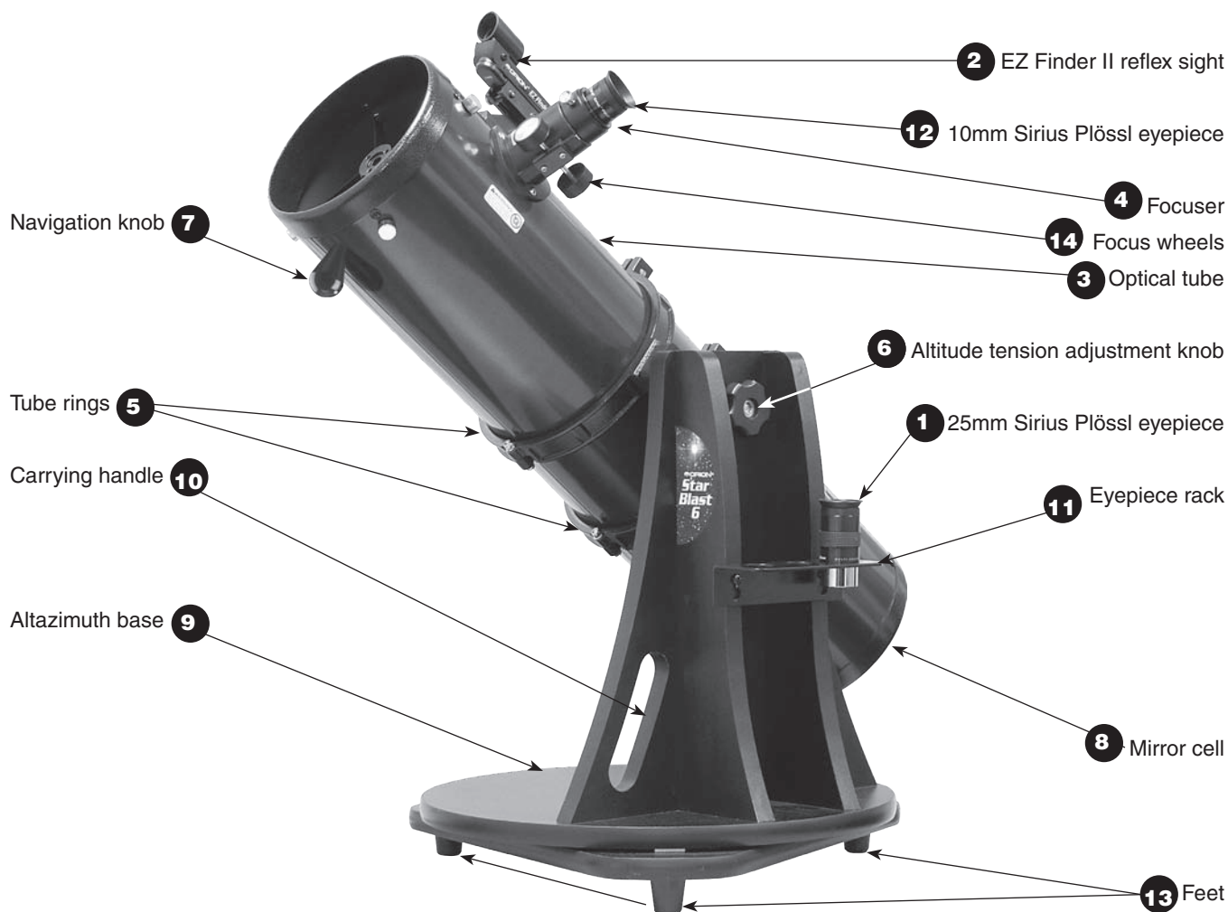
Figure 1. The StarBlast 6 Altazimuth Reflector
