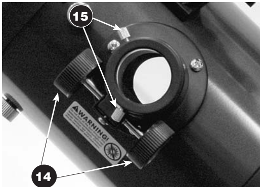
Figure 2. Details of the StarBlast 6 focuser.
