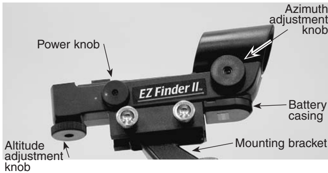
Figure 6. The EZ Finder II reflex sight.
