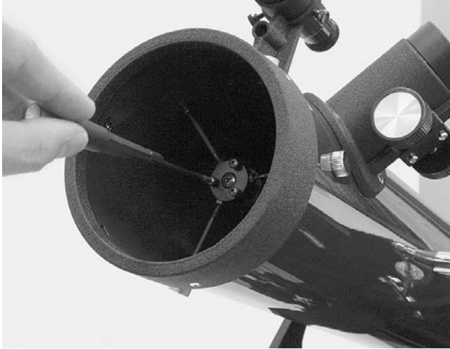
Figure 8. Adjust the tilt of the secondary mirror by loosening or tightening the three alignment screws with a small Phillips head screwdriver.
